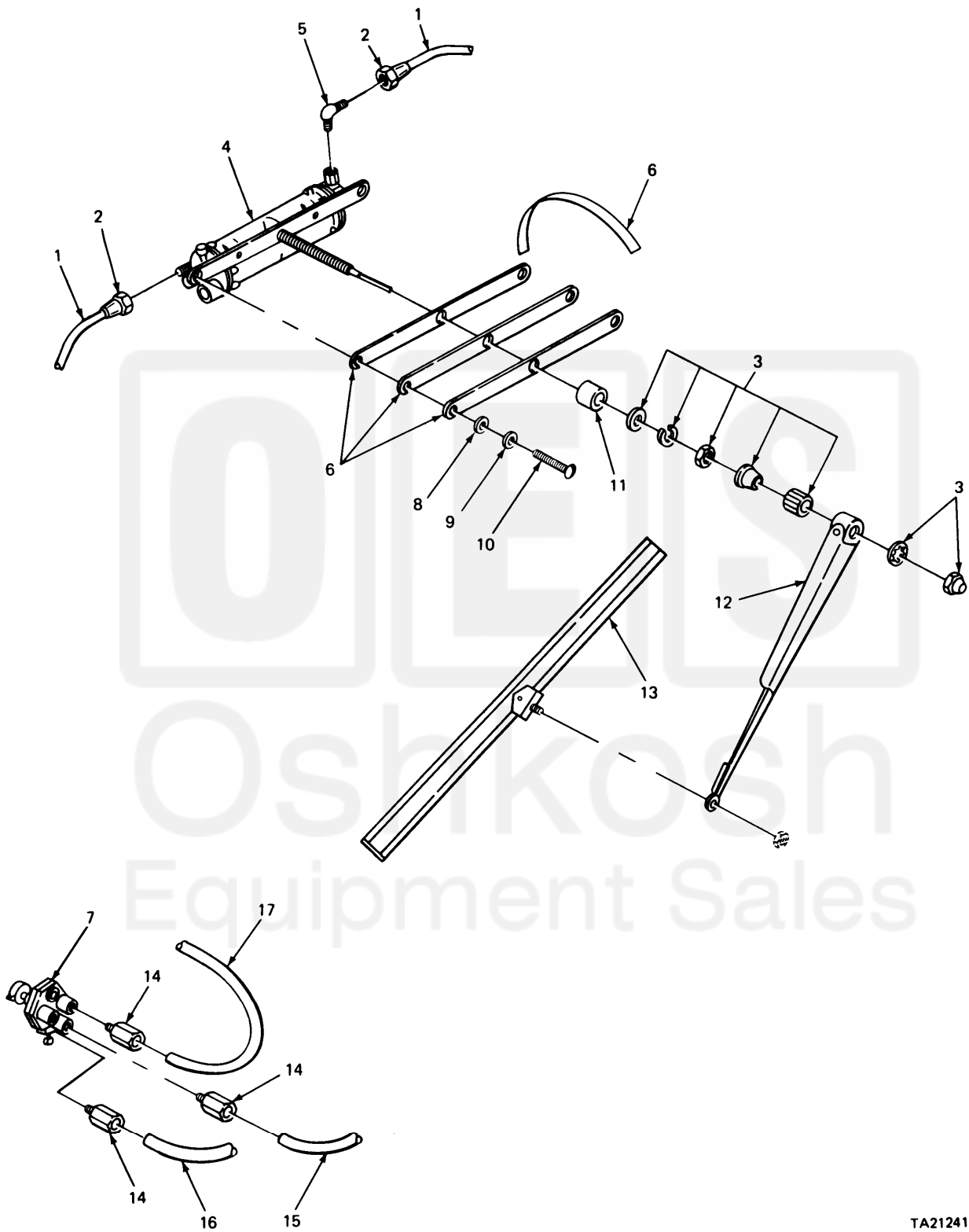
FIGURE 290. WIPER ASSEMBLY.
